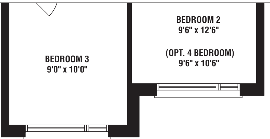
PARTIAL SECOND & OPT. SECOND FLOOR PLAN ELEV. 'C' (3 BEDROOM)
