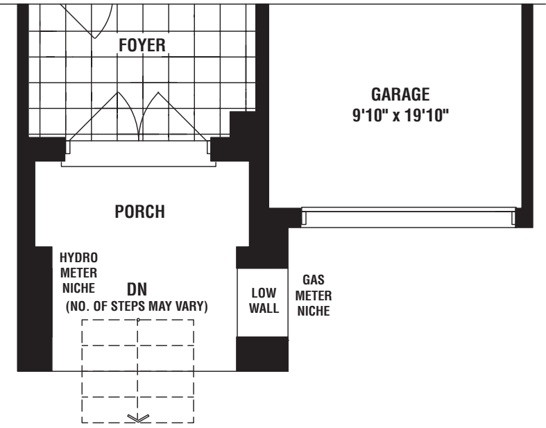
PARTIAL GROUND FLOOR PLAN ELEV. 'C'
