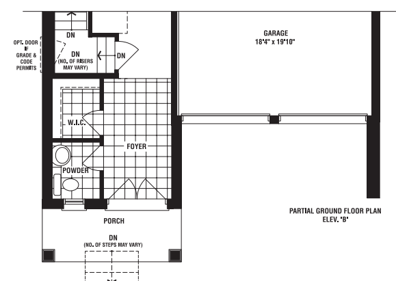
GROUND FLOOR PLAN ELEV. 'A'
