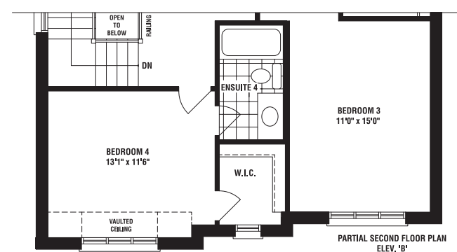
PARTIAL SECOND FLOOR PLAN
