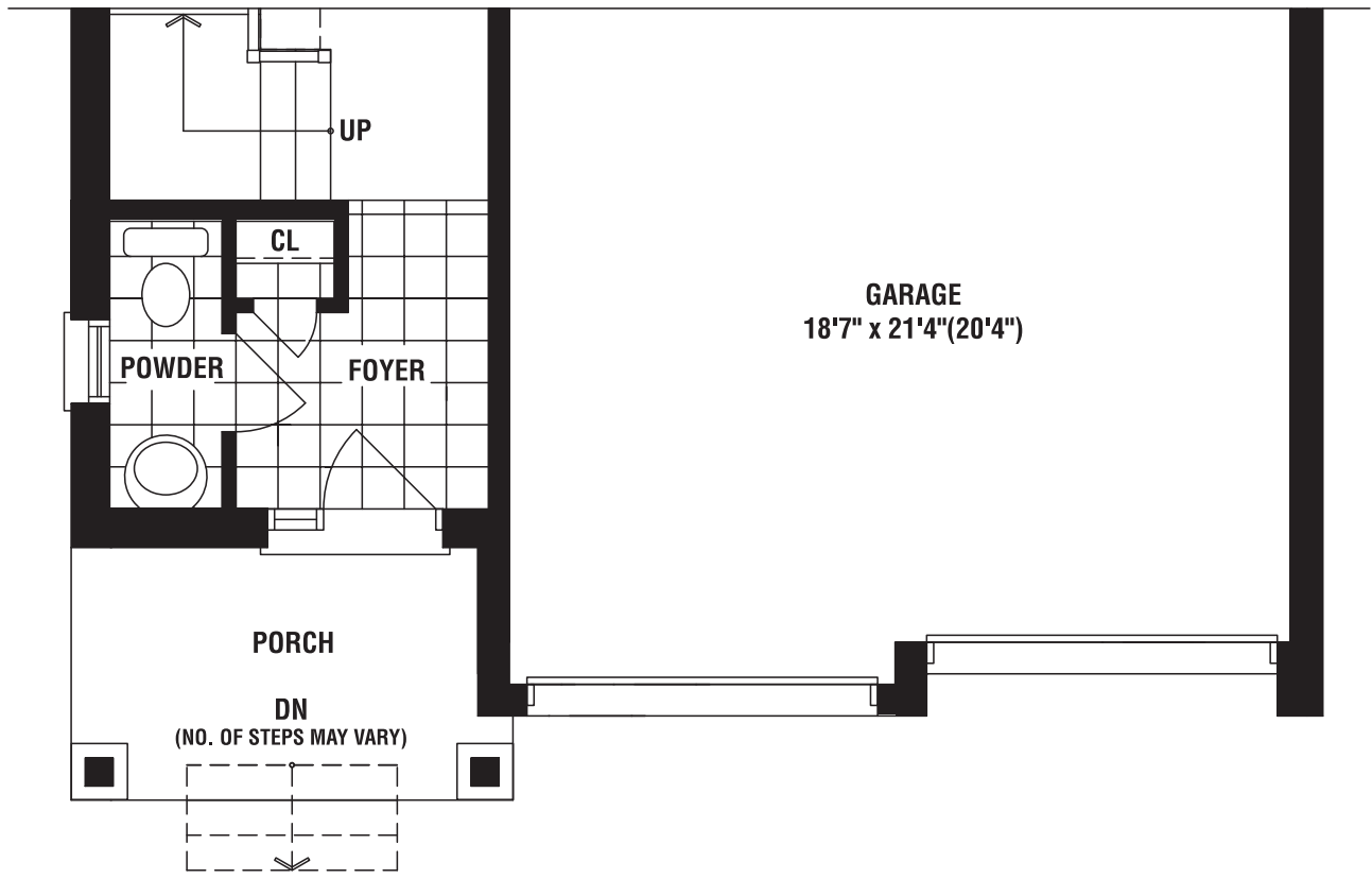
PARTIAL GROUND FLOOR PLAN ELEV. 'C'
