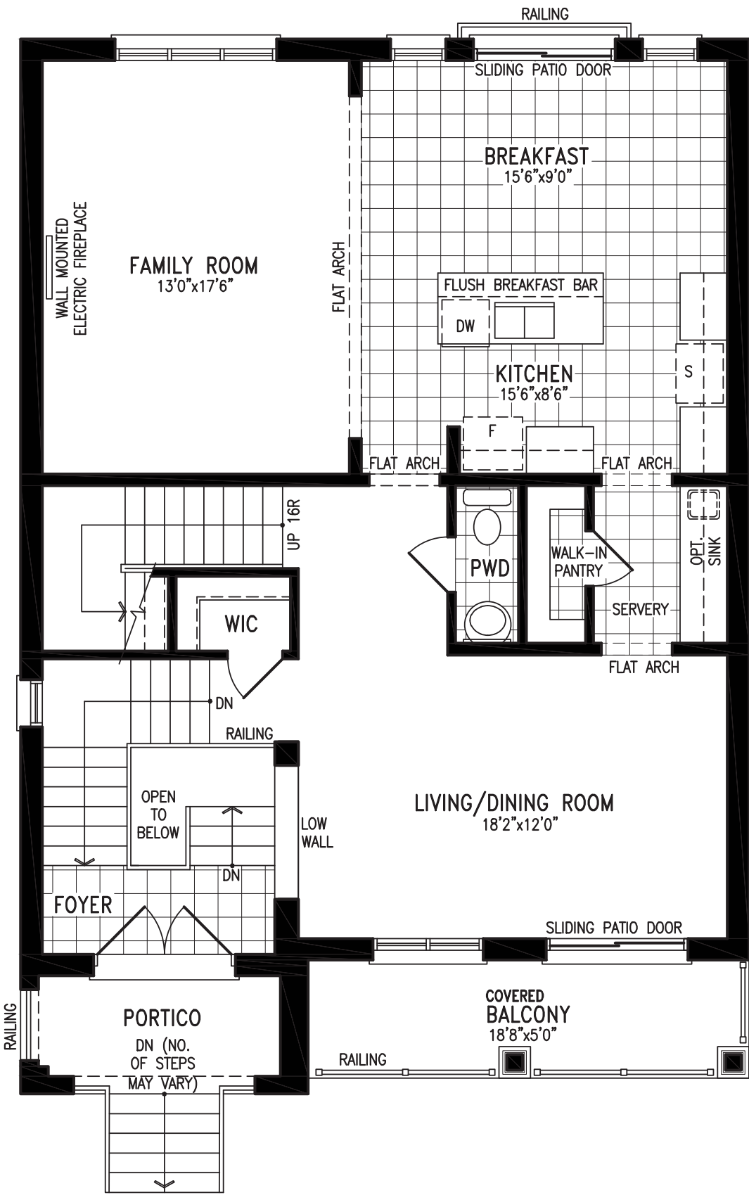
MAIN LEVEL PLAN ELEV. 'A'
