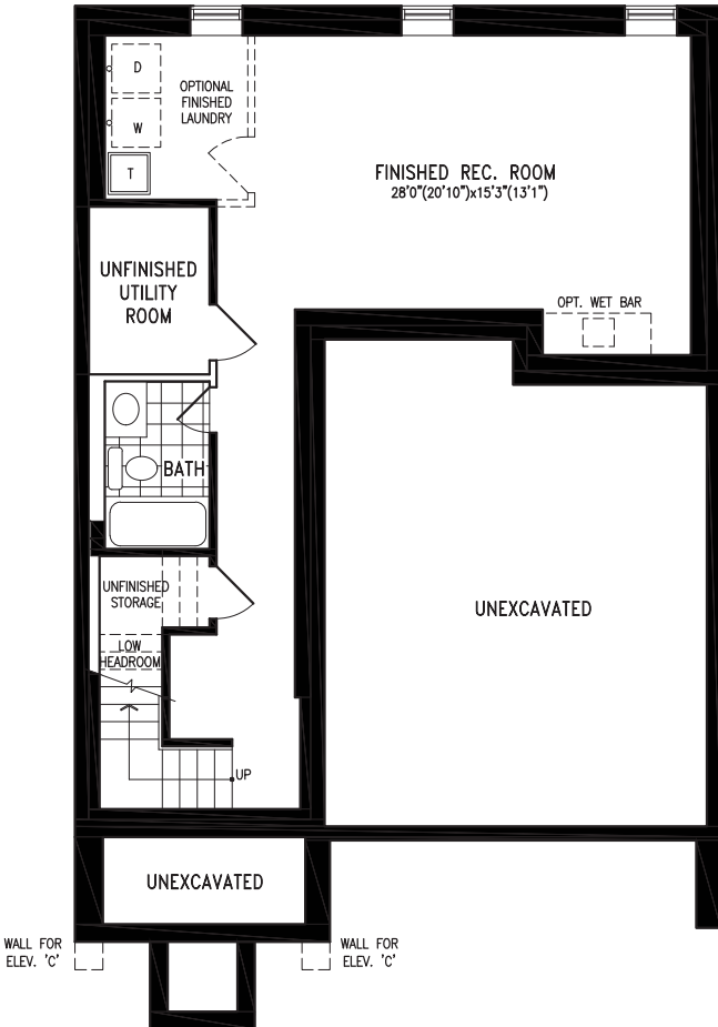
OPT. FINISHED BASEMENT PLAN ELEV. 'A' & 'C' (OPT. FIN. BASEMENT: 'A'/'C' 615 SF)
