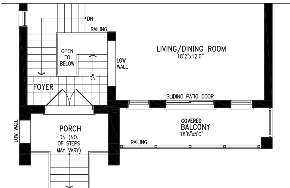
PARTIAL MAIN LEVEL PLAN ELEV. 'C'
