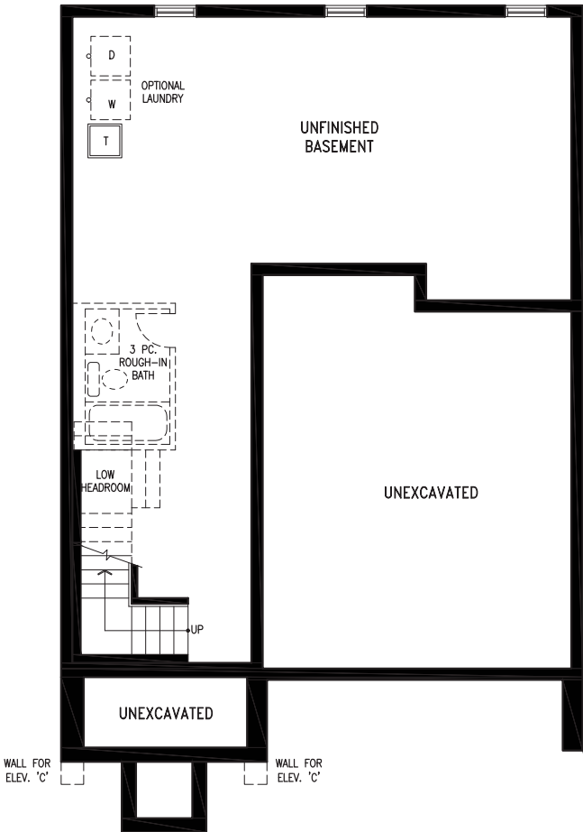
BASEMENT PLAN ELEV. 'A' & 'C'
