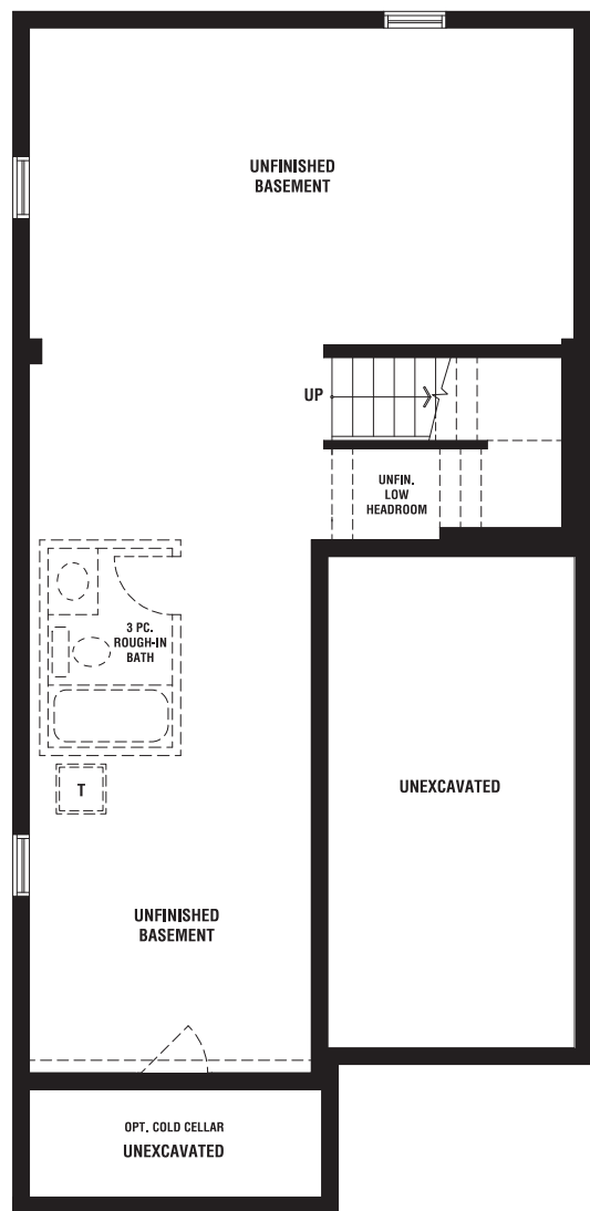
BASEMENT PLAN ELEV. 'A'
