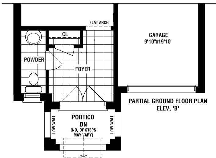
PARTIAL OPT. GROUND FLOOR PLAN WALK-UP CONDITION
