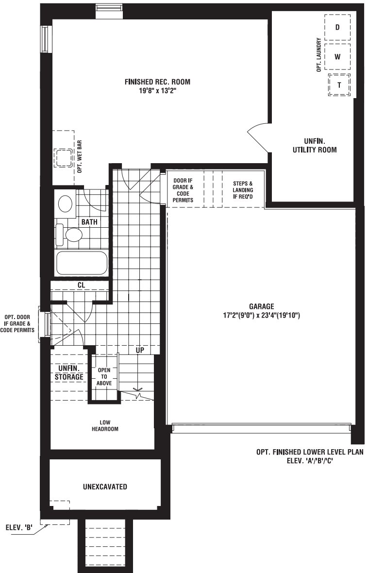
LOWER LEVEL PLAN ELEV. 'A'/B'/C'
