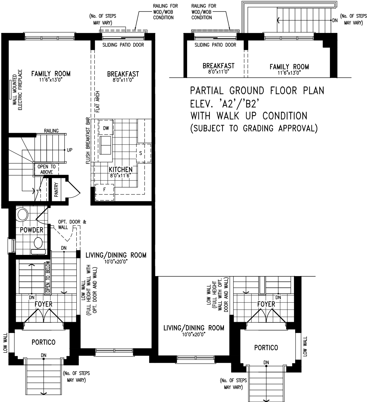
GROUND FLOOR PLAN ELEV. 'A1'
