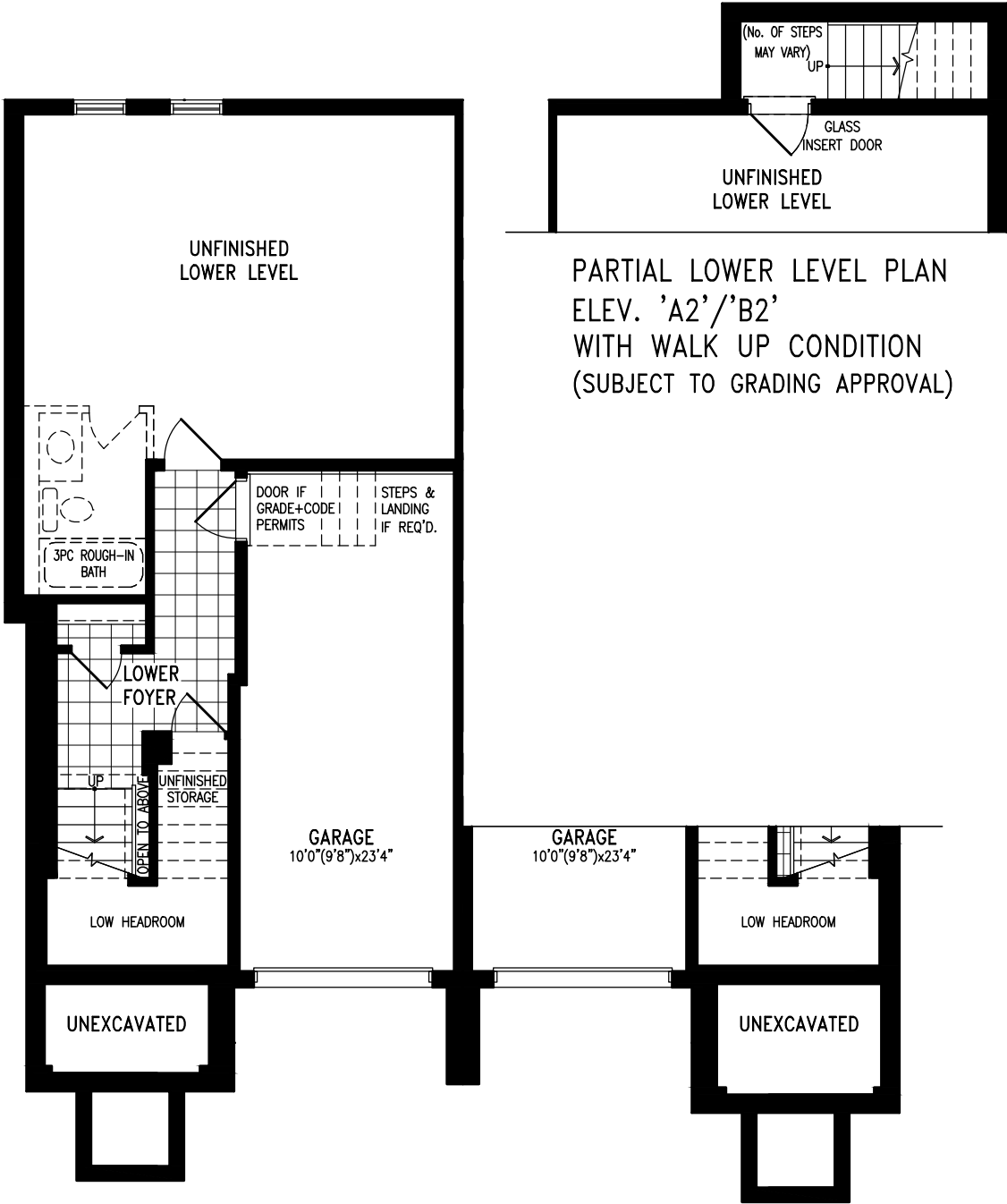
LOWER LEVEL PLAN ELEV. 'A1'
