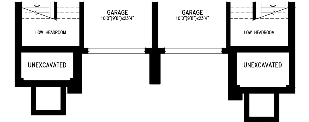
PARTIAL LOWER LEVEL PLAN ELEV. 'B1'
