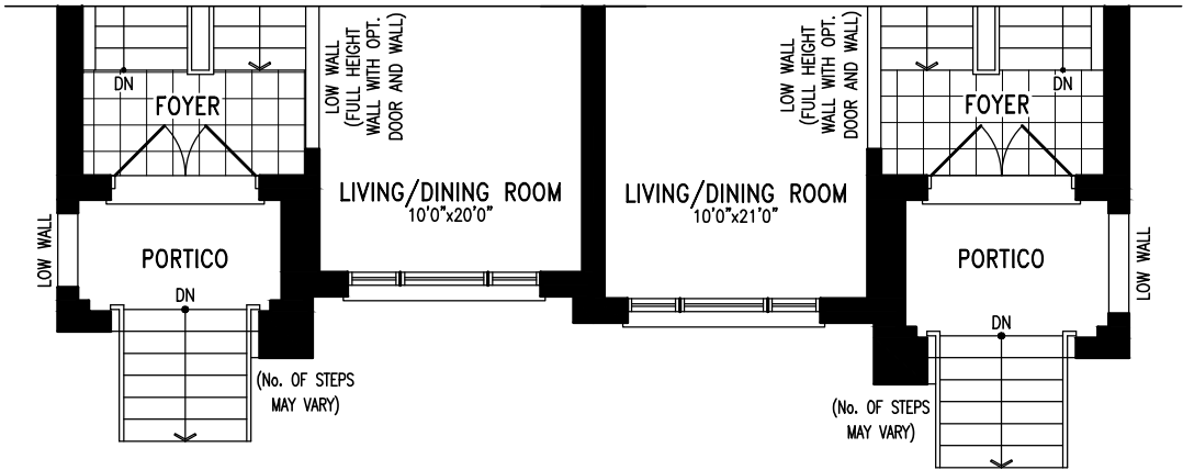
PARTIAL GROUND FLOOR PLAN ELEV. 'B1'
