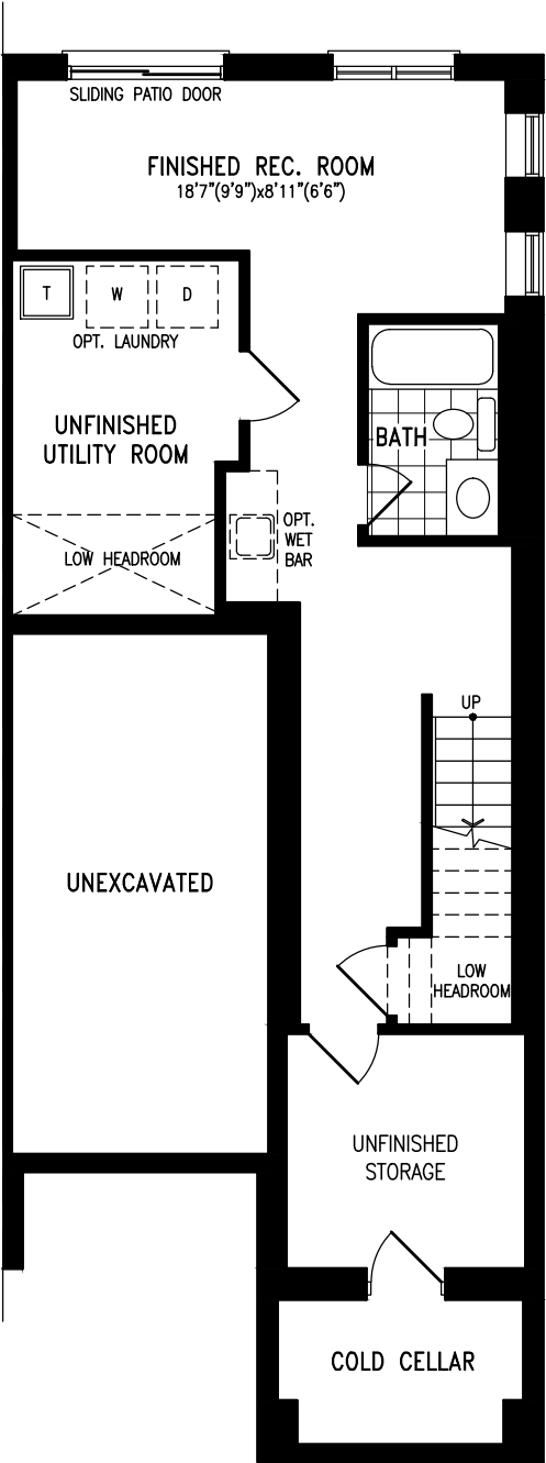
OPTIONAL FINISHED BASEMENT PLAN ELEV. 'A2' (LOT:109R)
