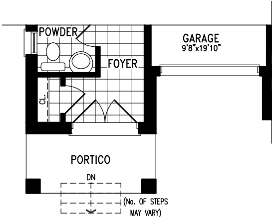
GROUND FLOOR PLAN ELEV. 'B1' (LOT:20L)
