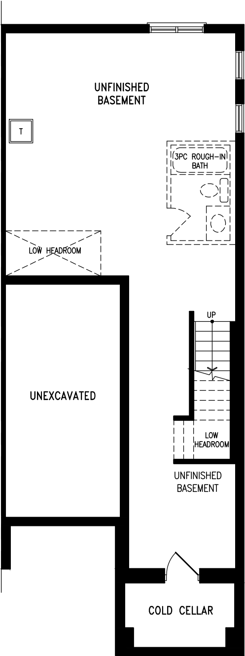
BASEMENT PLAN ELEV. 'A2' (LOT:109R)
