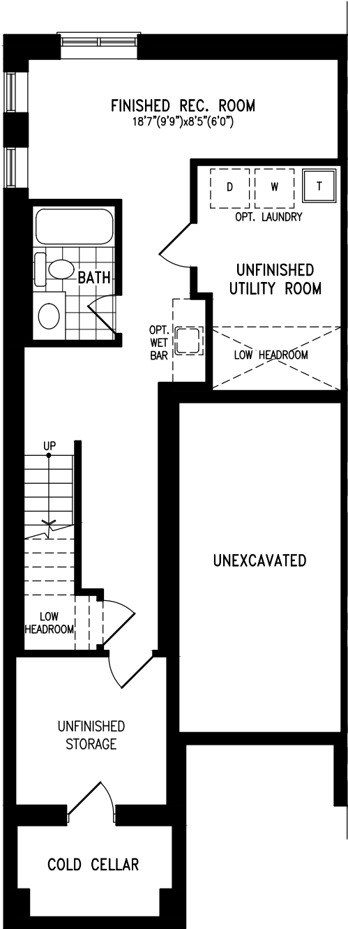
OPTIONAL FINISHED BASEMENT PLAN ELEV. ‘A1’ (LOT:20L)
