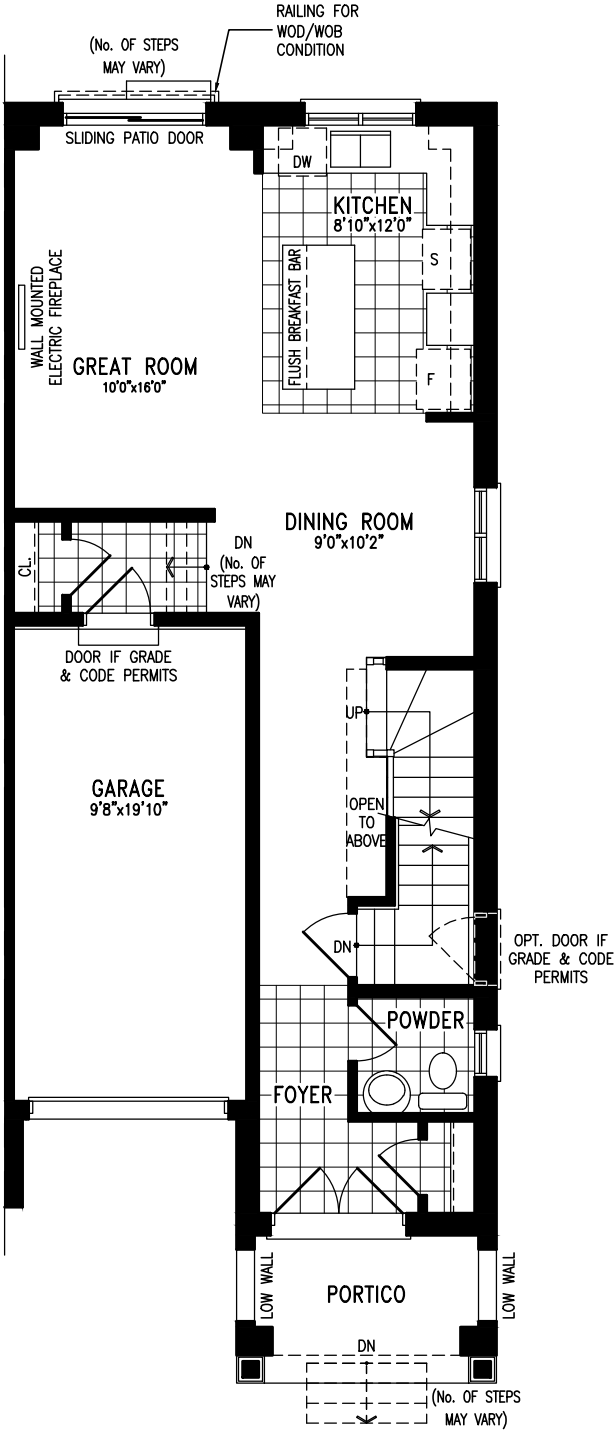
GROUND FLOOR PLAN ELEV. 'A2' (LOT:109R)
