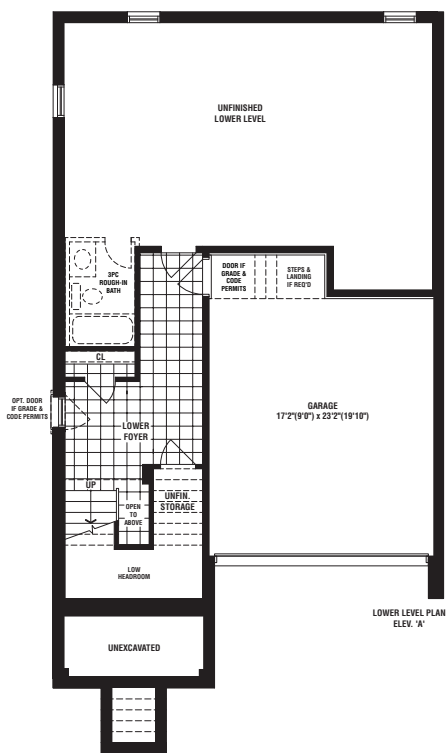
LOWER LEVEL
