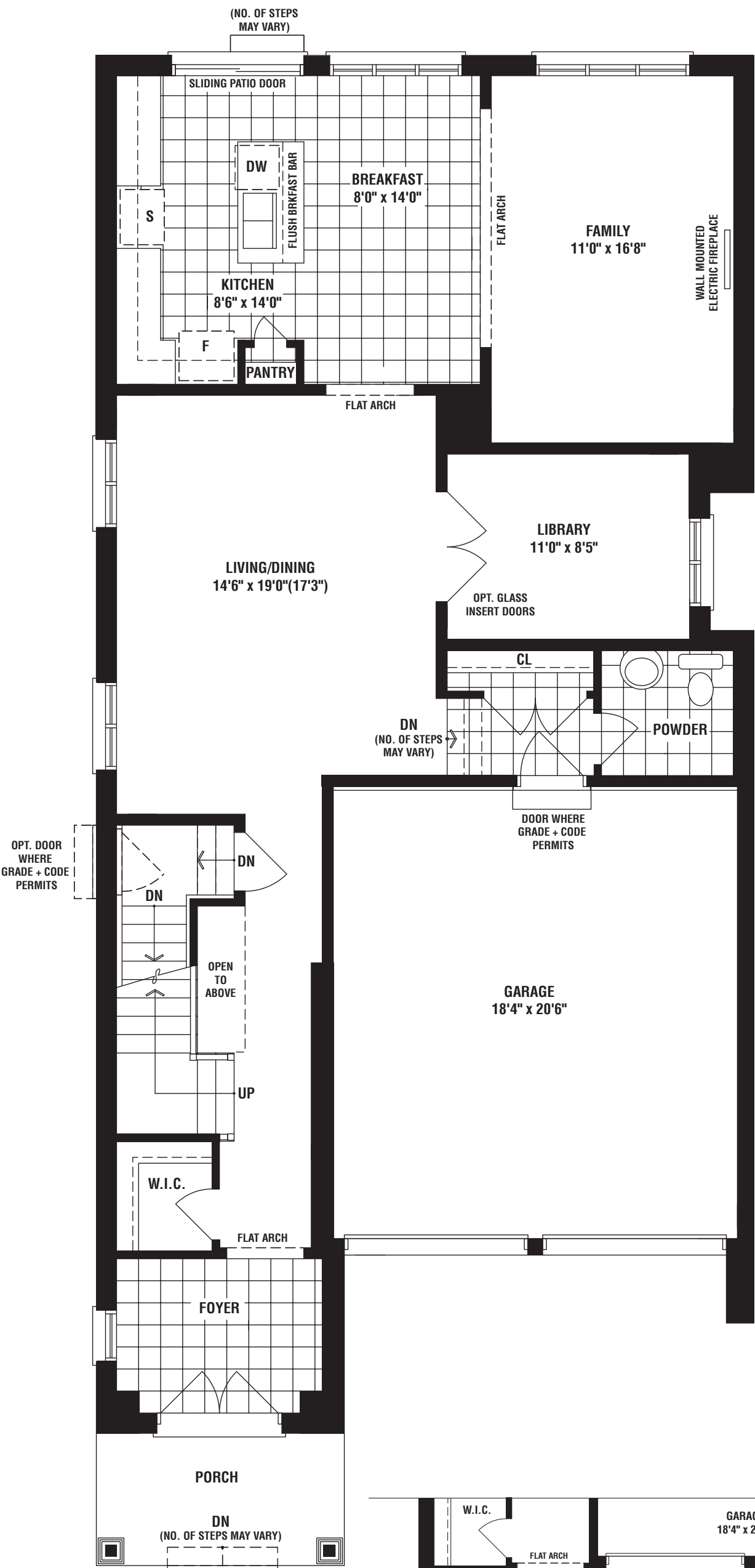
GROUND FLOOR PLAN ELEV. 'A'
