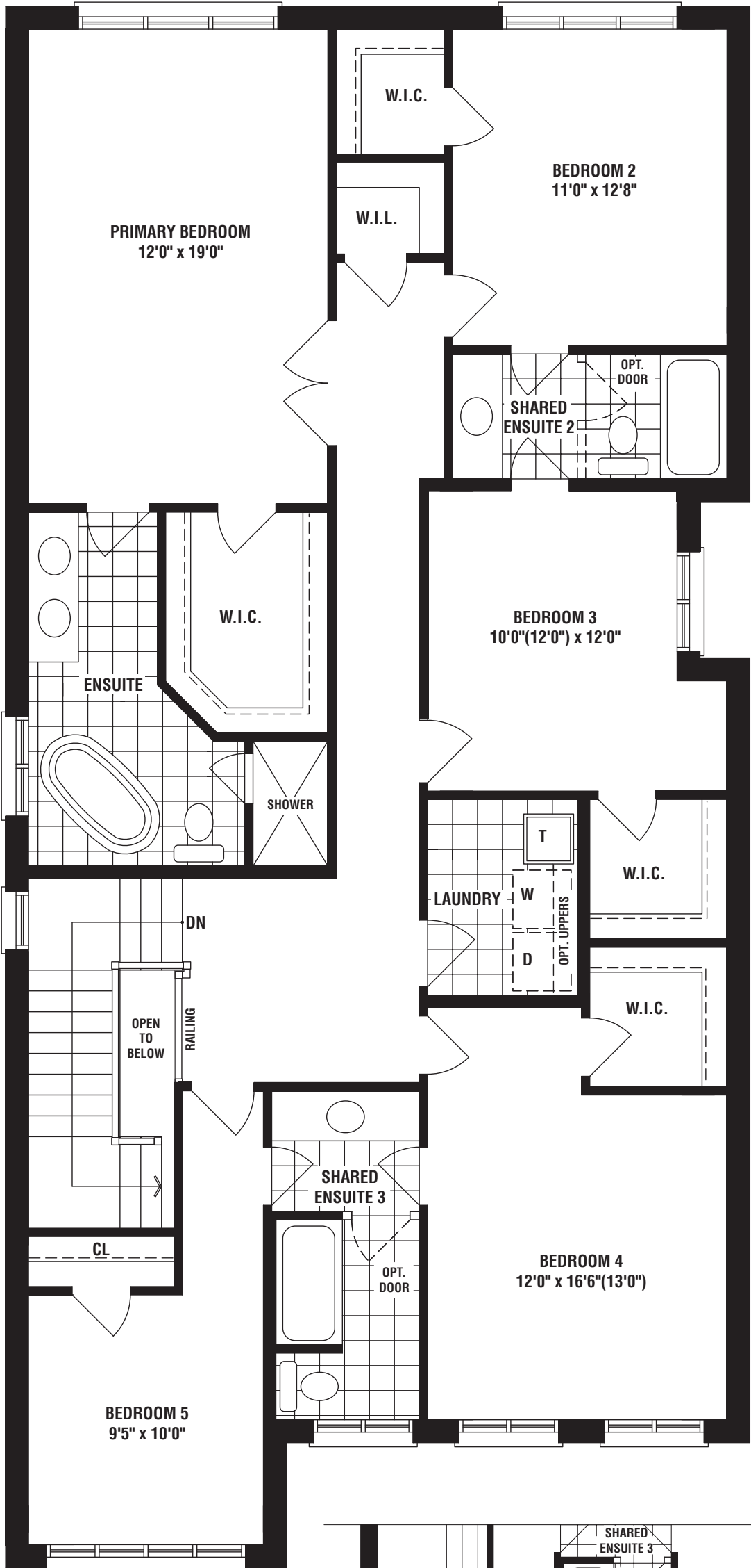
SECOND FLOOR PLAN ELEV. 'A'
