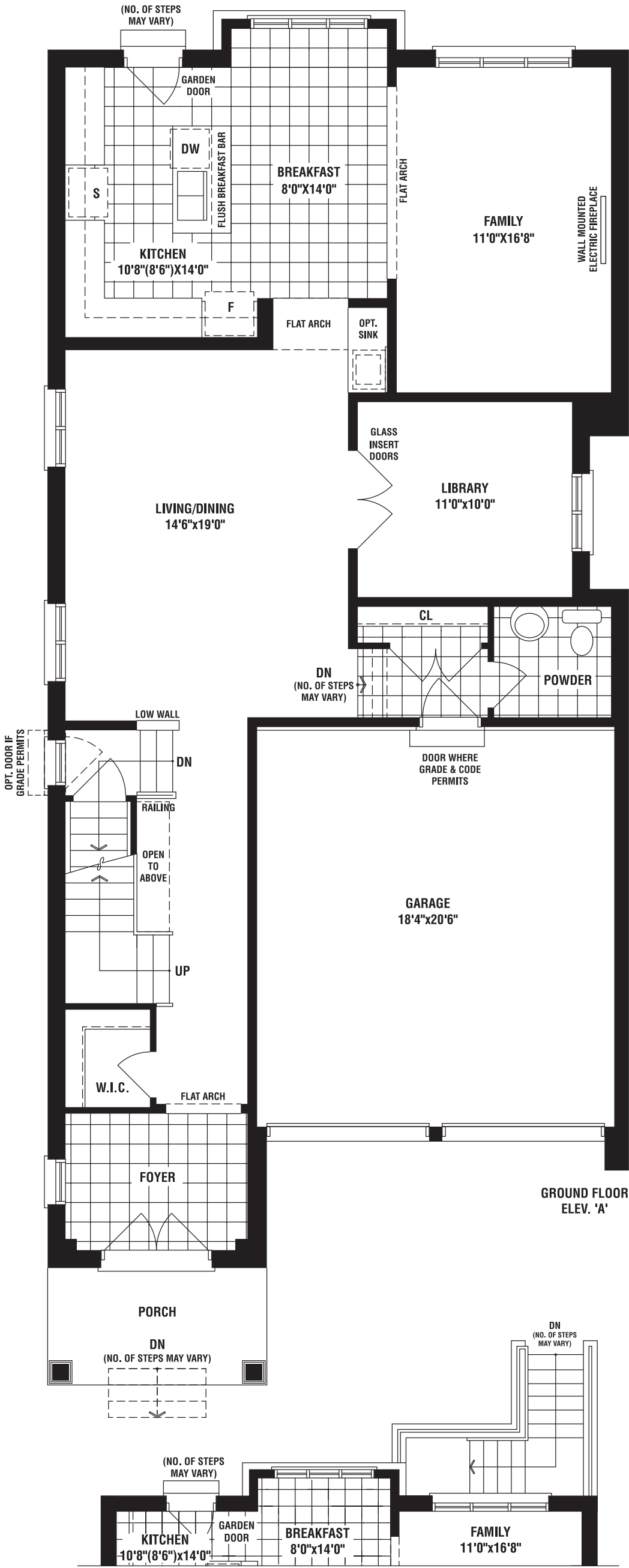
PARTIAL GROUND FLOOR PLAN OPT. WALK UP BASEMENT CONDITION (SUBJECT TO GRADING APPROVAL) (LOCATION MAY VARY)
