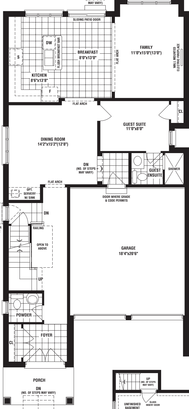
OPT. GROUND FLOOR (GUEST SUITE) ELEV. 'A'
