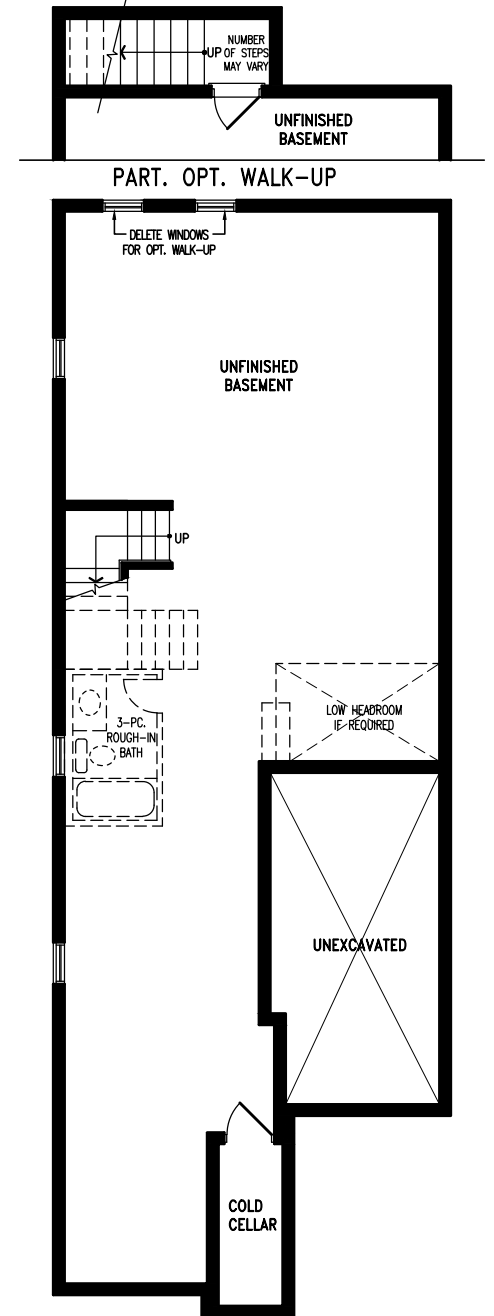
BASEMENT PLAN ELEV. 'A' & 'B'
