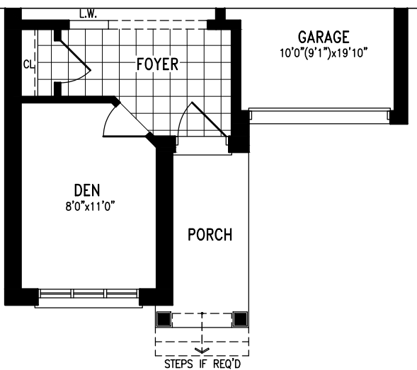
PART. GROUND FLOOR PLAN ELEV. 'B'
