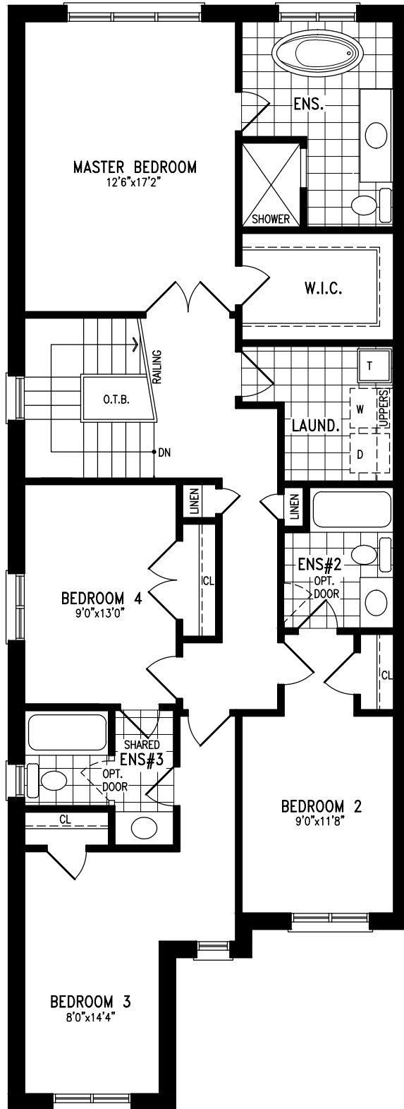
SECOND FLOOR PLAN ELEV. 'A'
