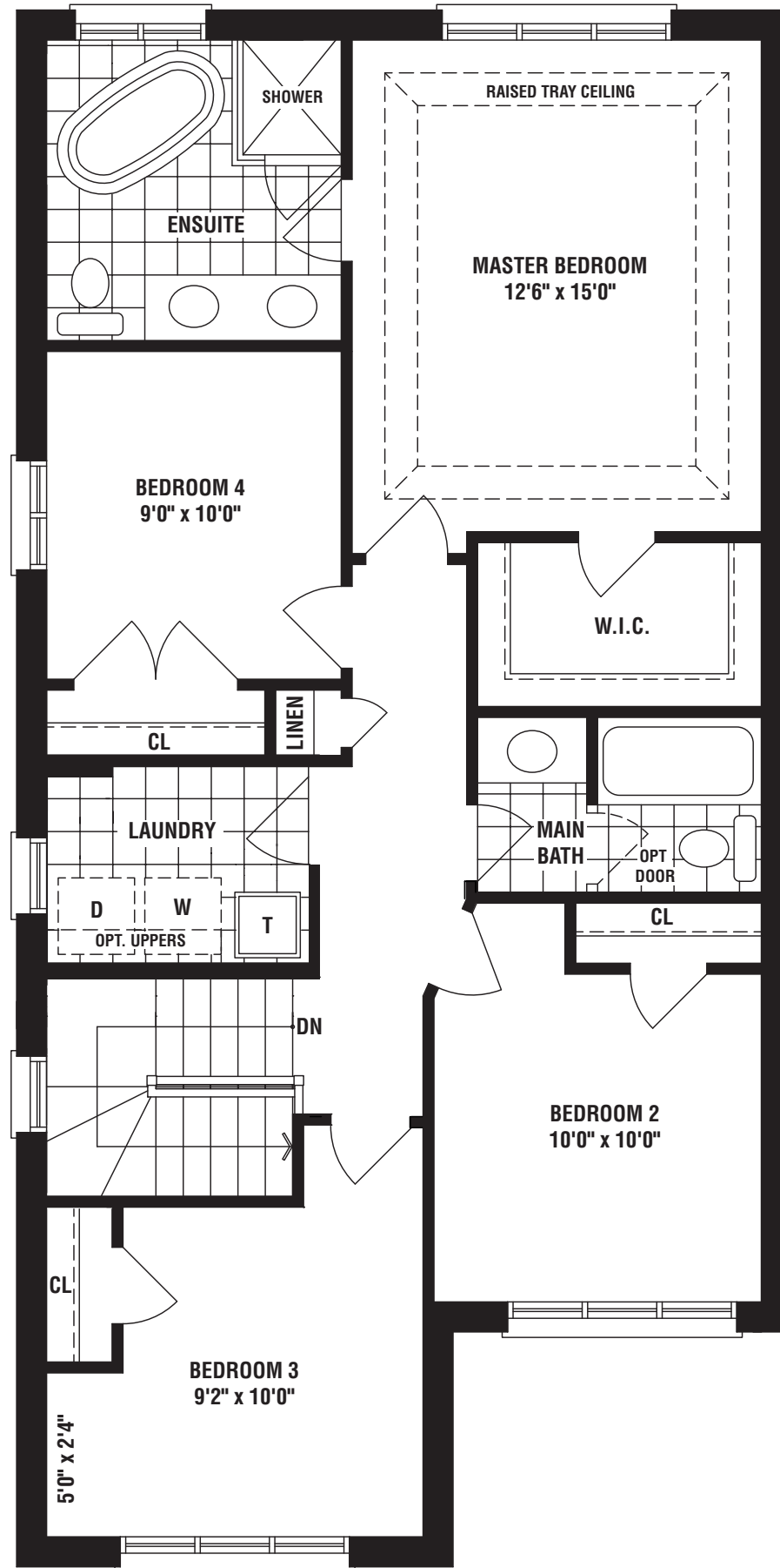
SECOND FLOOR PLAN ELEV. 'A' 4 BEDROOM
