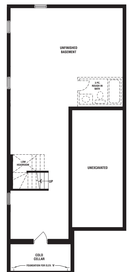
BASEMENT PLAN ELEV. 'A' & 'B'
