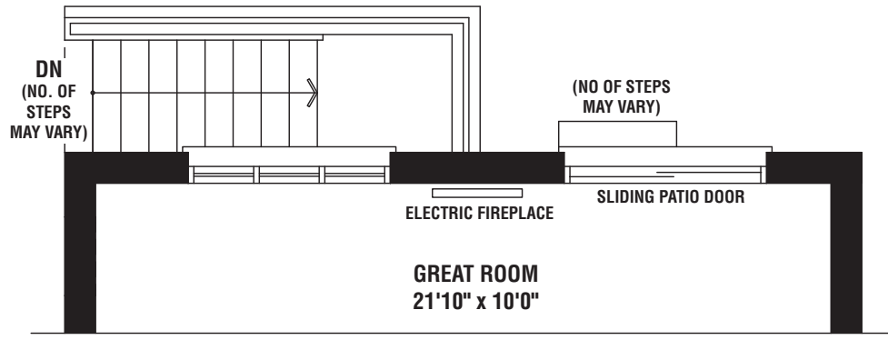
PARTIAL GROUND FLOOR PLAN WALK-UP CONDITION (SUBJECT TO GRADING APPROVAL)
