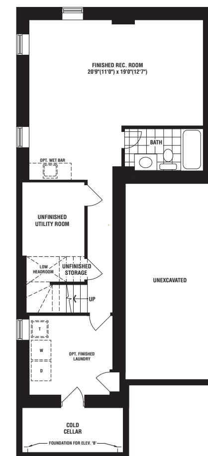
OPT. FINISHED BASEMENT PLAN ELEV. 'A' & 'B' (OPT. FIN. BASEMENT: 10'0\"/>
