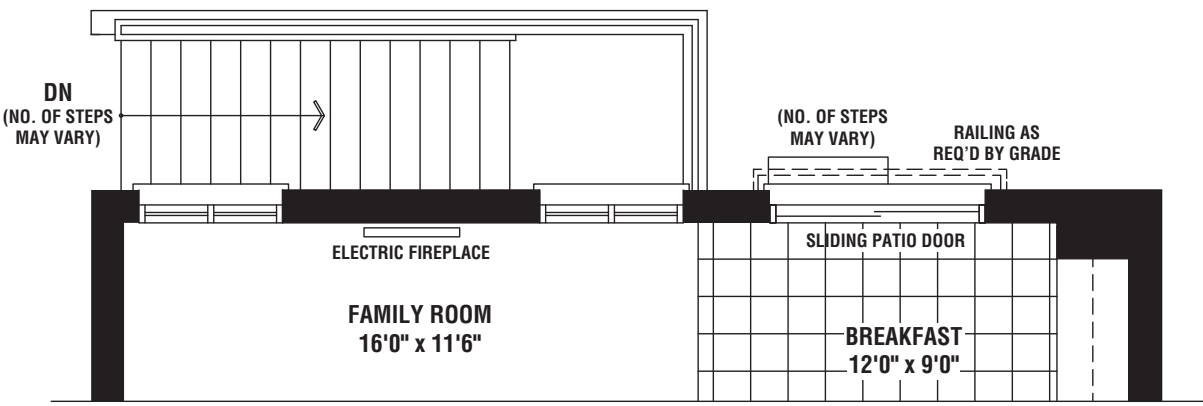
PARTIAL GROUND FLOOR PLAN WALK-UP CONDITION (SUBJECT TO GRADING APPROVAL)
