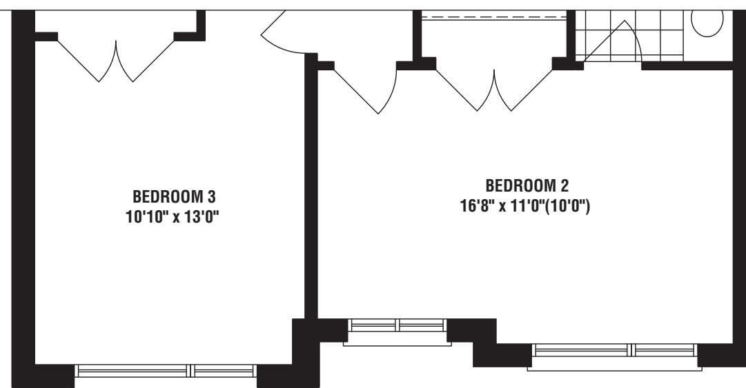
PARTIAL SECOND FLOOR PLAN ELEV. 'B'
