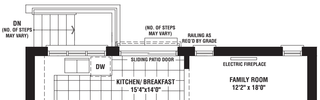
PARTIAL GROUND FLOOR PLAN WALK-UP CONDITION (SUBJECT TO GRADING APPROVAL)
