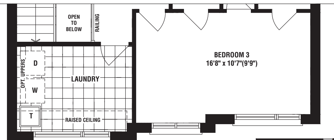
PARTIAL SECOND FLOOR PLAN ELEV. 'B' (5 BEDROOM SIMILAR)
