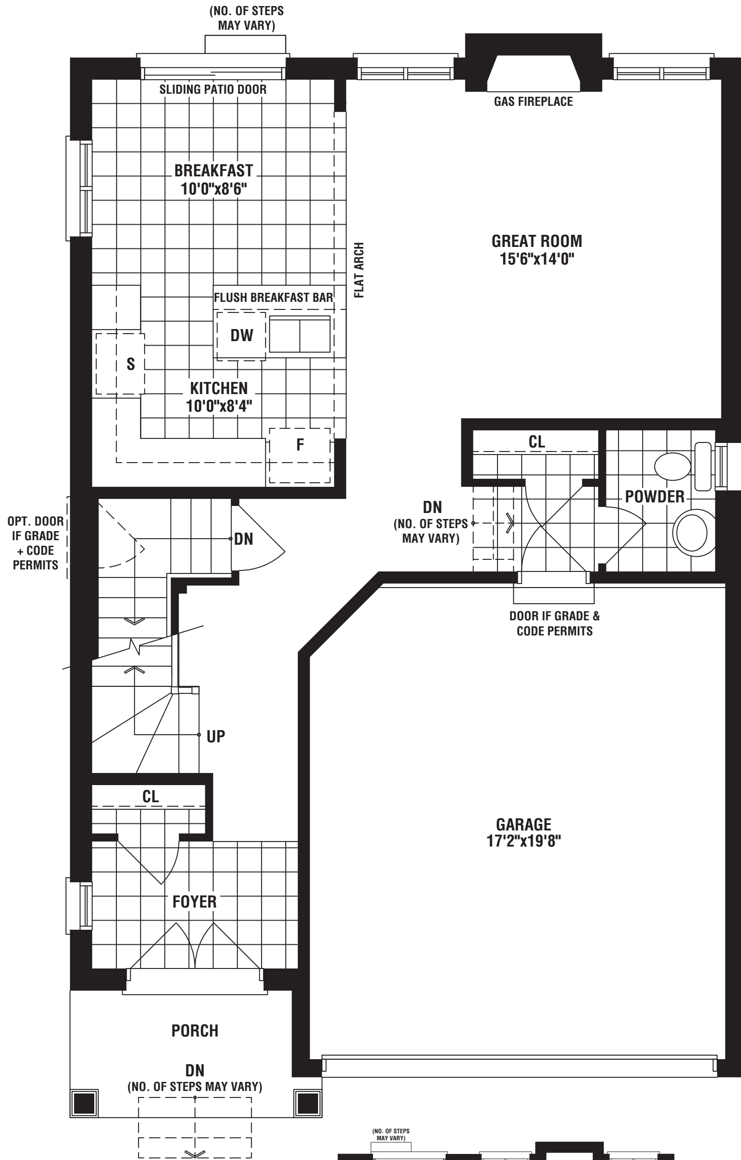
GROUND FLOOR PLAN ELEV. 'A'
