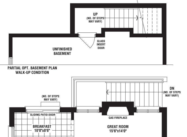
PARTIAL OPT. GROUND FLOOR PLAN WALK-UP CONDITION
